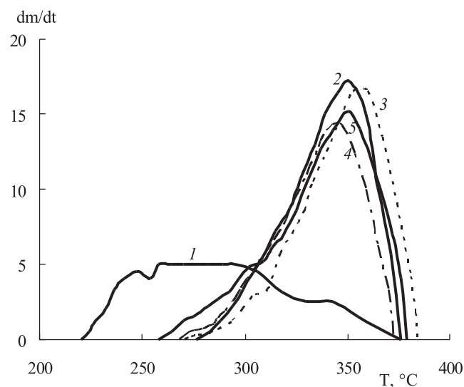
Figure 5. DTG curves of PMMA synthesized at 60°C in the presence of AIBN (1.0 mmol/l) ( 1 ), AIBN and porphyrin 2 (1.0 mmol/l) ( 2-5 ). Monomer conversion, %: 20 ( 1 , 2 ); 40 ( 3 ); 60 ( 4 ) and 80 ( 5 ).
