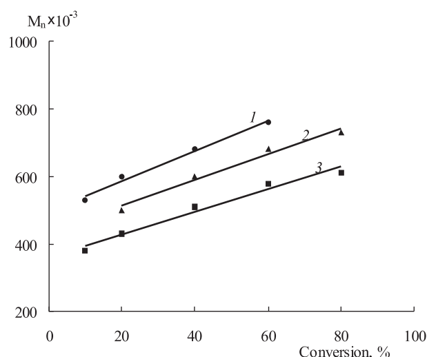
Figure 2. M_n of PMMA obtained in the presence of AIBN (1.0 mmol/l) and porphyrins 1 ( 1 ), 2 ( 2 ) and 3 ( 3 ) (1.0 mmol/l) vs. monomer conversion. Polymerization temperature is 60°C.
