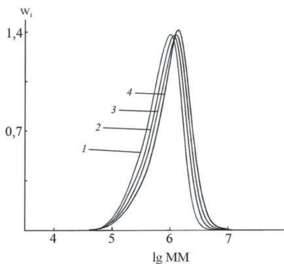
Figure 4. MWD curves of PMMA obtained in the presence of AIBN (1.0 mmol/l) and porphyrin 1 (1.0 mmol/l) at 60°C. Monomer conversion, %: 10 ( 1 ), 20 ( 2 ), 40 ( 3 ), 60 ( 4 ). w_i – mass fraction of macromolecules with certain molecular mass (MM).
