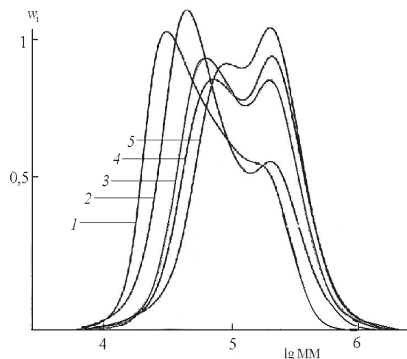
Figure 9. MWD curves of PMMA obtained in the presence of benzoyl peroxide (1.0 mmol/l) and porphyrin 4 (0.5 mmol/l). Monomer conversion, %: 3 (1), 8 (2), 10 (3), 20 (4), 60 (5). Polymerization temperature is 60°C. w_i – mass fraction of macromolecules with certain molecular mass (MM).
