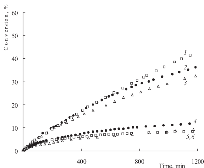
Figure 8. Conversion vs. MMA polymerization time at 60°C in the presence of AIBN and porphyrins 4 (3), 5 (2) and 6 (1); benzoyl peroxide (1.0 mmol/l) and porphyrins (1.0 mmol/l) 4 (5), 5 (4) and 6 (6).
